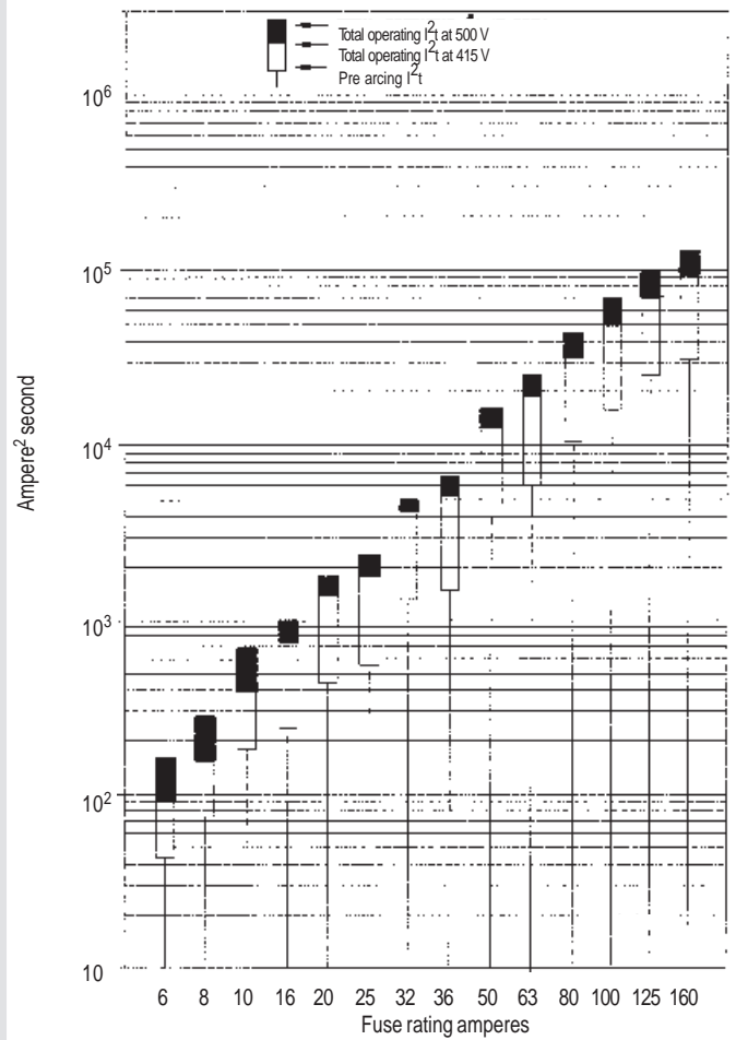
I^2t characteristics
